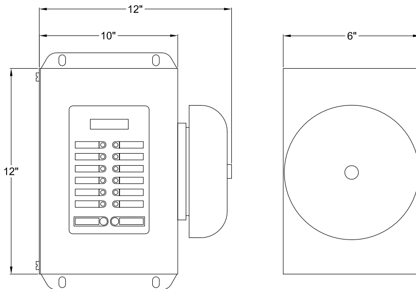
NEMA 1 ENCLOSURE FINISHED FIRE RED
