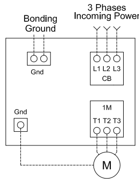
Circuit Breaker (CB) Field Wiring according to Bending Space (AWG or MCM). TERMINALS L1 - L2 - L3
