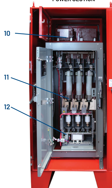
POWER SECTION
