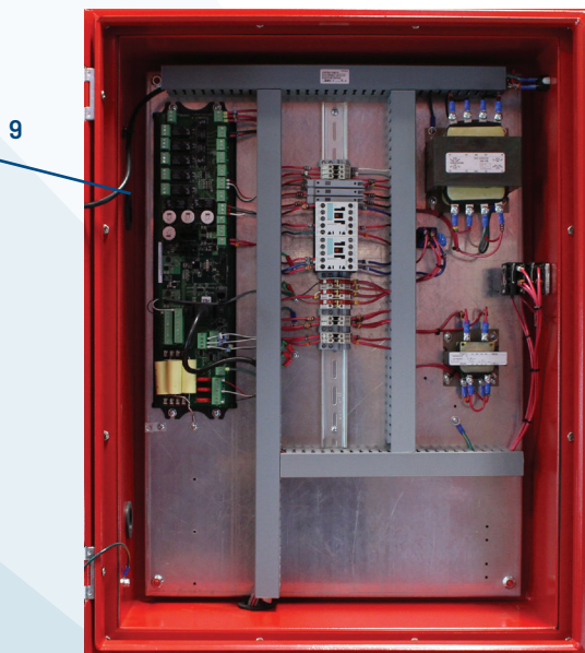
CONTROL SECTION
