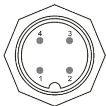
Fig. 2 Electrical connection
