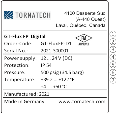
Fig. 1 Type plate, GT-FluxFP Digital measuring transducer
