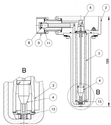
Fig. 1 GT-FluxFP orifice plate and bypass meter, Drawing and dimensions 2"/DN 50 - 4"/DN 100
