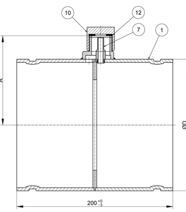
Fig. 2 GT-FluxFP orifice plate, Drawing and dimensions 6"/DN 150 - 12"/DN 300
