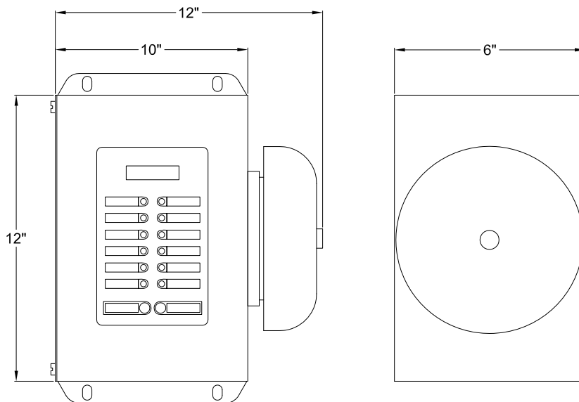
NEMA 1 ENCLOSURE RED RAL 3002
